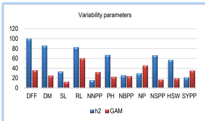
Fig-2 Heritability and genetic advance as percent of mean of given population
